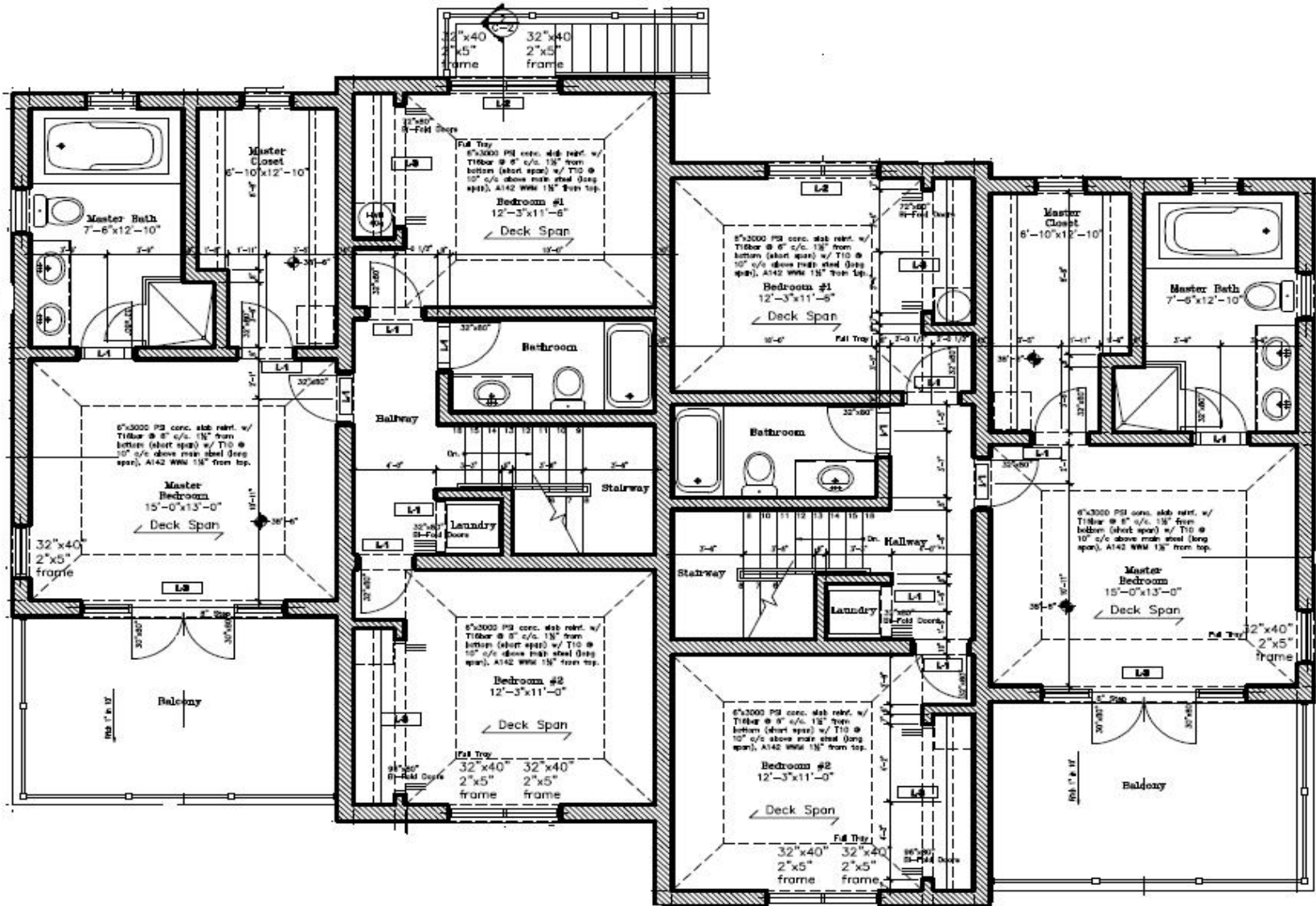
SECOND FLOOR LEVEL
