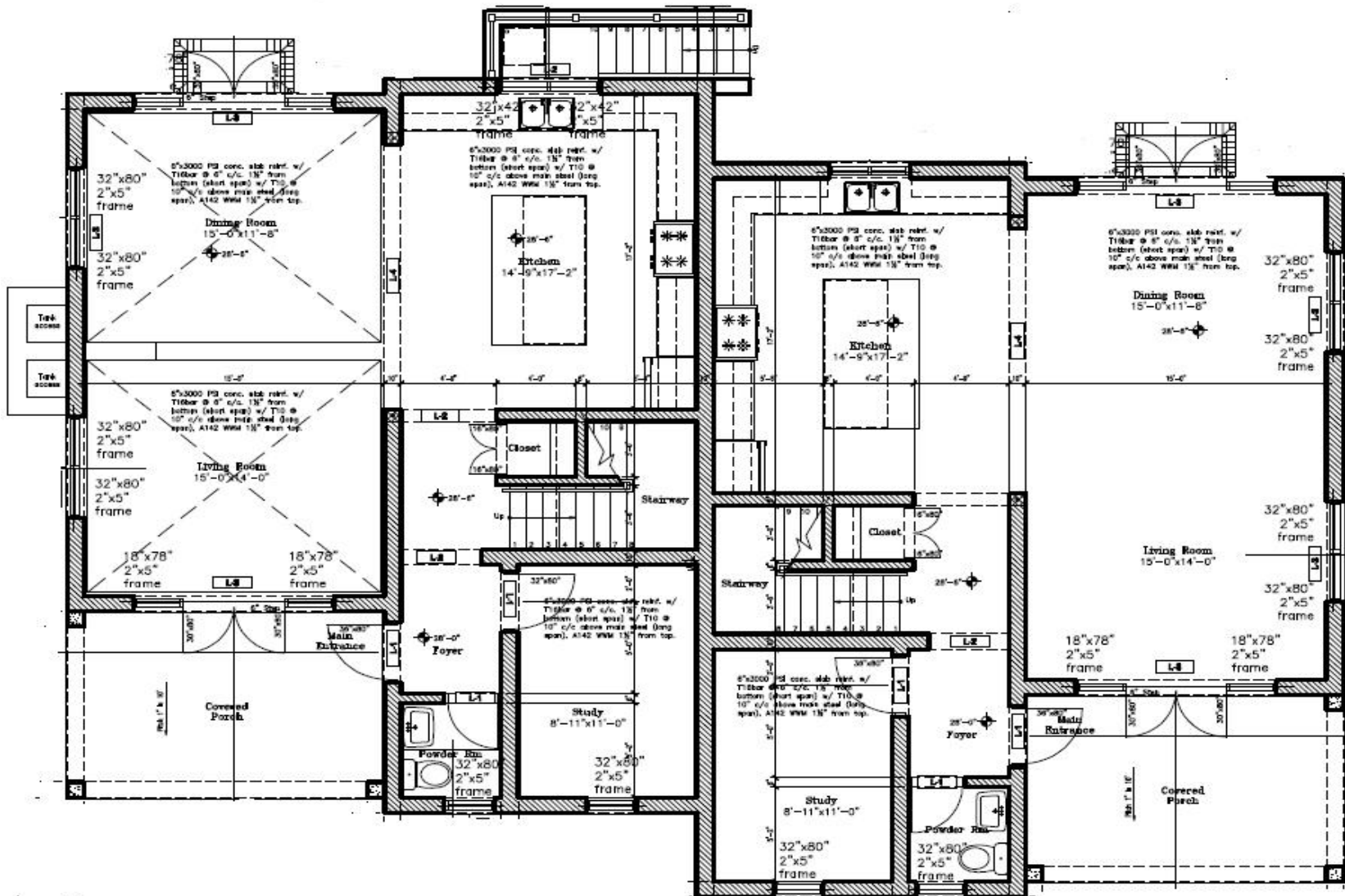
GROUND FLOOR LEVEL
